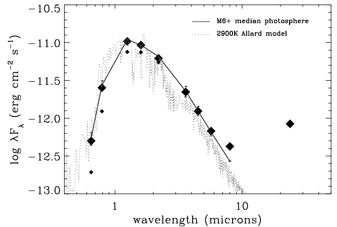
FIG. 3.—Observed SED for the substellar object L316 ( diamonds ). Ground-based optical and near-infrared photometry are taken from Luhman et al. (2003), IRAC data from Lada et al. (2006) and Luhman et al. (2005). All fluxes have been dereddened using the observed A_V and the reddening law of Mathis (1990) ( large diamonds ); the original reddened fluxes are also shown ( small diamonds ). The median SED and 1\sigma dispersion for 8 IC 348 members with spectral types later than M6 which lack infrared excess, normalized to the L316 SED at J , are shown with the solid line and error bars (from Lada et al. 2006). For further comparison, a photospheric model with T_{\text{eff}} = 2900 K from Allard et al. (2001) is shown with the dotted line. Note the systematically lower flux of this model compared to the empirical photosphere at the first 3 IRAC bands, which might cause a false inference of excess emission if one relied only on the model to represent the intrinsic substellar photosphere. [See the electronic edition of the Journal for a color version of this figure.]
