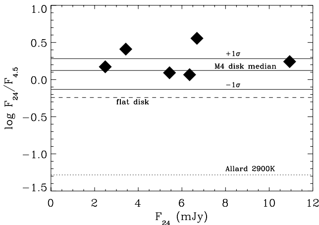
FIG. 2.—Ratio of fluxes at 24 and 4.5 \mu\text{m} as a function of the 24 \mu\text{m} flux for the six low-mass/substellar 24 \mu\text{m} detections ( filled diamonds ), all dereddened using A_V determined empirically from optical photometry and spectral types (Luhman et al. 2003) and the Mathis (1990) reddening law. The theoretical flux ratio for an M6.5 photosphere, derived from an Allard et al. (2001) AMES-COND model for T_{\text{eff}} = 2900 K, is shown with the dotted line. The dashed line shows the flux ratio upper limit for a spectral slope \lambda F_\lambda \propto \lambda^{-4/3} corresponding to a geometrically thin, optically thick flat disk, assuming negligible contribution to the 4.5 \mu\text{m} flux from the photosphere. The solid line shows the median slope, and the dot-dashed lines show the \pm 1\sigma values for \sim 15 members of IC 348 with spectral types M4–M5 with excesses indicative of optically thick disks, as defined in Lada et al. (2006).
