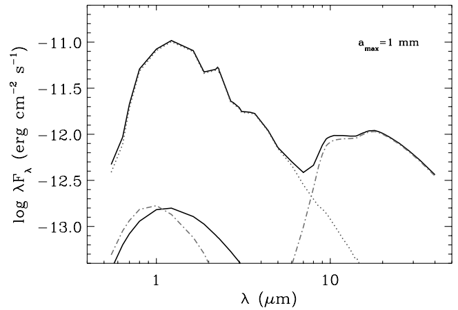
FIG. 6.—Same as in Fig. 5 with a_{\max} = 1 \text{ mm} for the case of a large ( \sim 1 \text{ AU} ) inner disk hole. [See the electronic edition of the Journal for a color version of this figure.]
